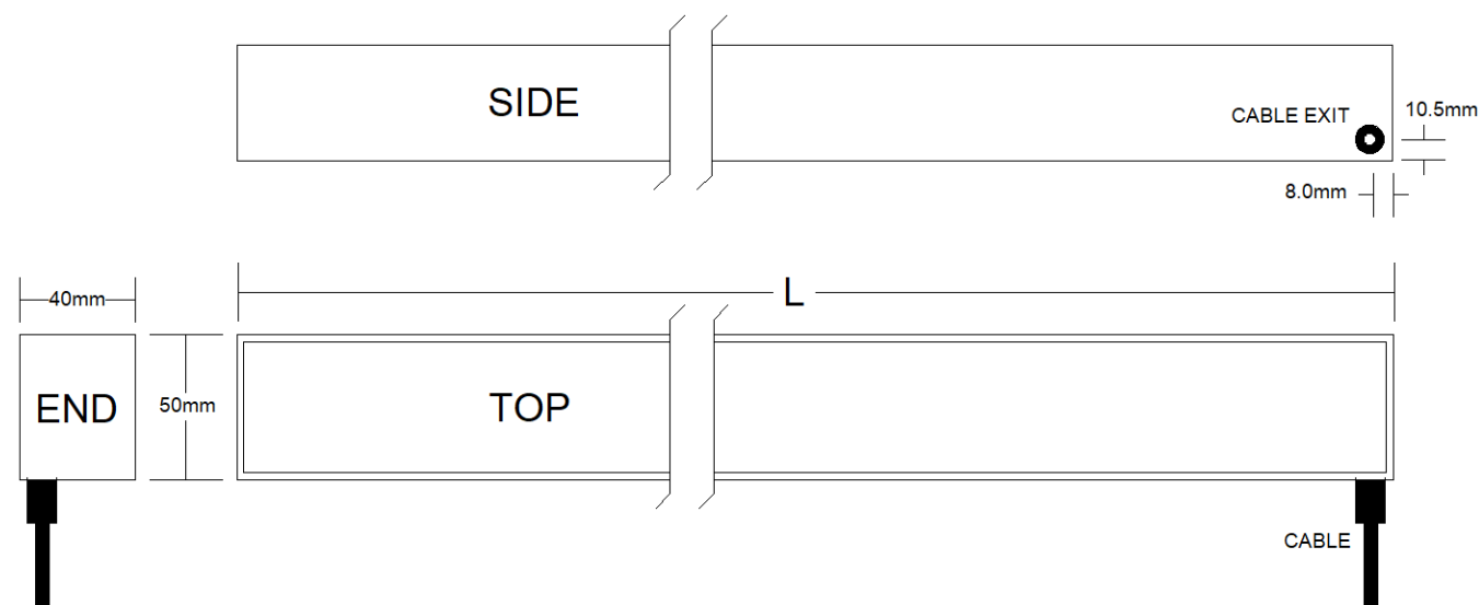
Figure 1. Outline Dimensions
